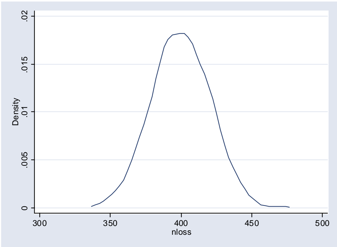
Figure 3: N=100,000 ; 1,000 replications
