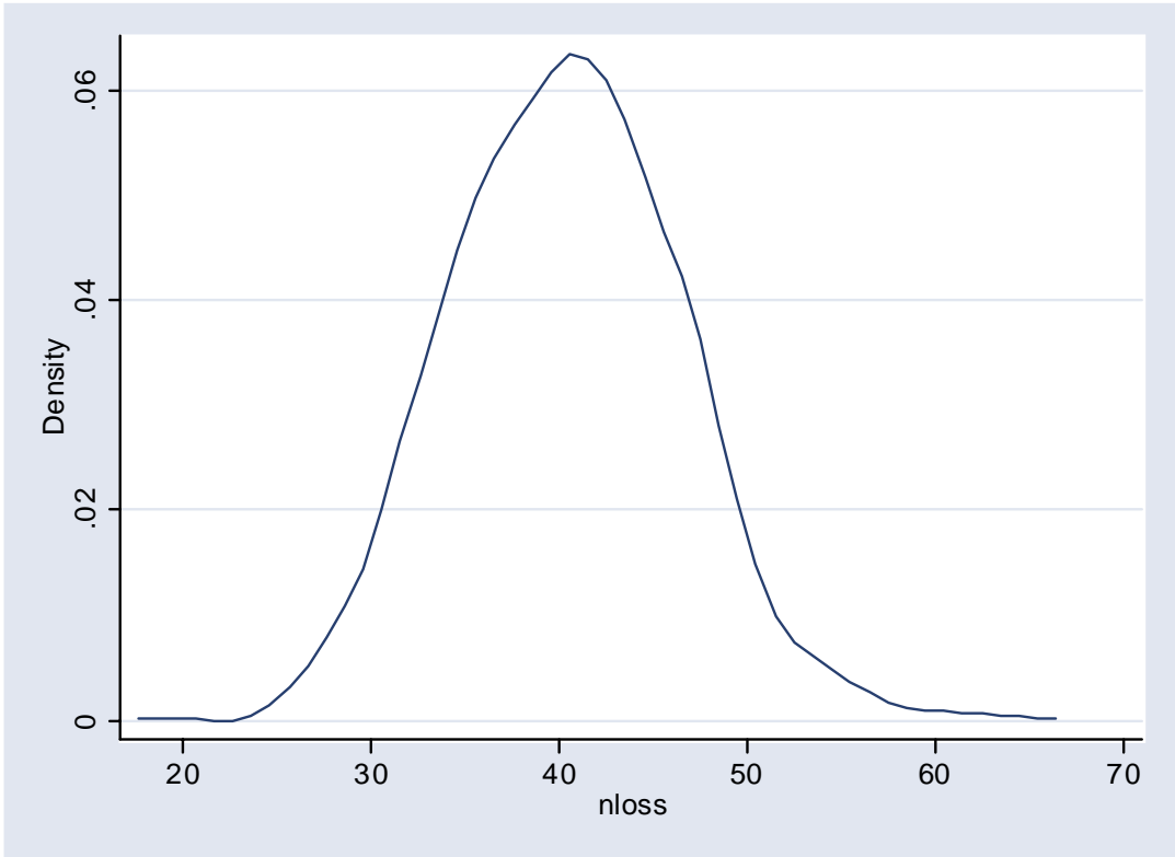
Figure 2: N=10,000 ; 1,000 replications
