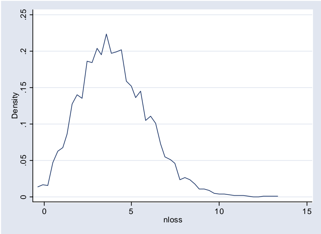
Figure 1: N=1,000; 1,000 replications
