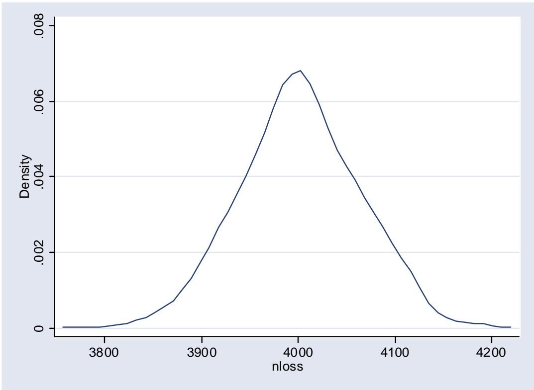
Figure 4: N=1,000,000 ; 1,000 replications
