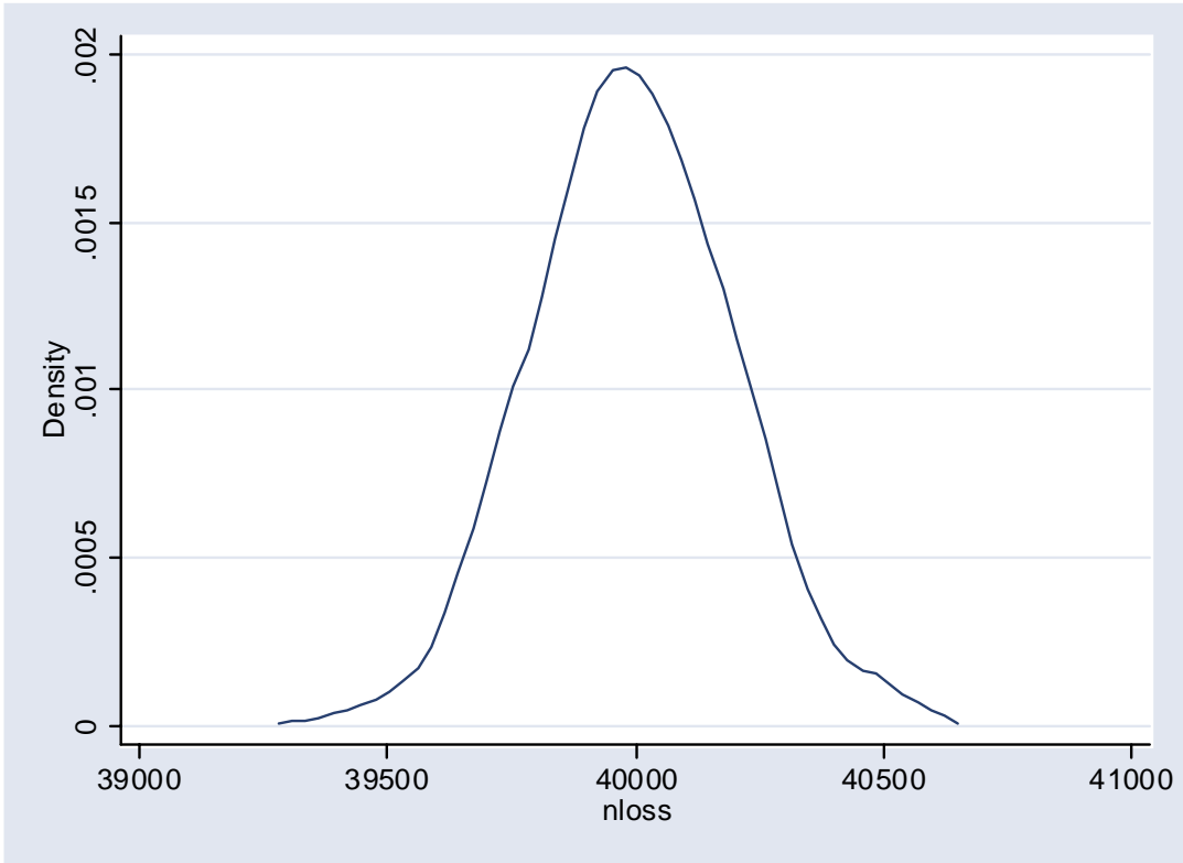
Figure 5: N=10,000,000 ; 1,000 replications
